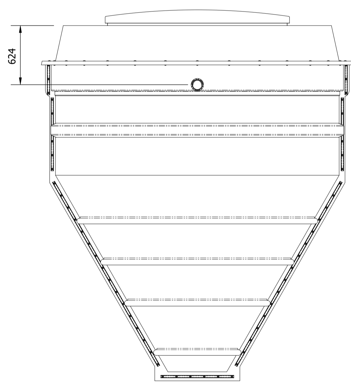
OUTLET VIEW
