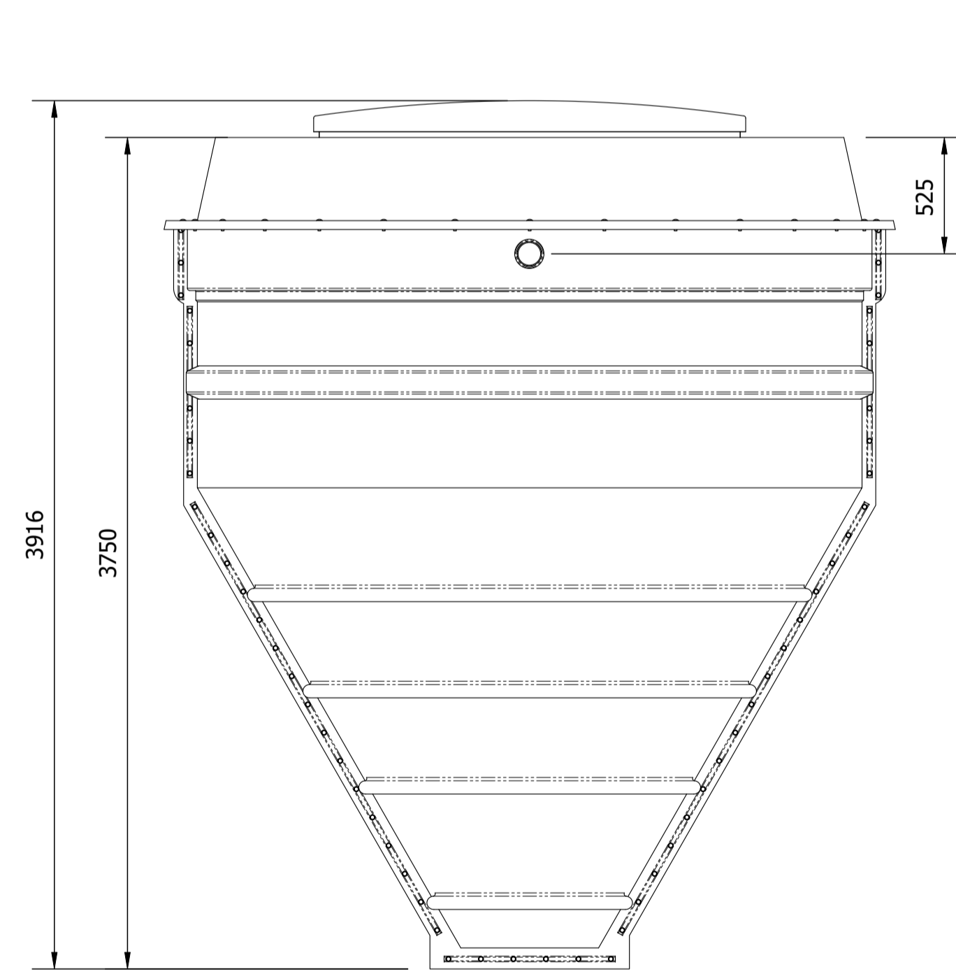
INLET VIEW
