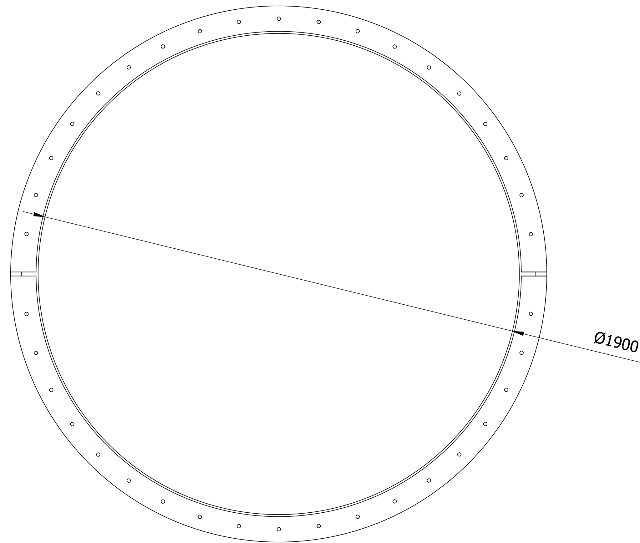
PLAN VIEW
