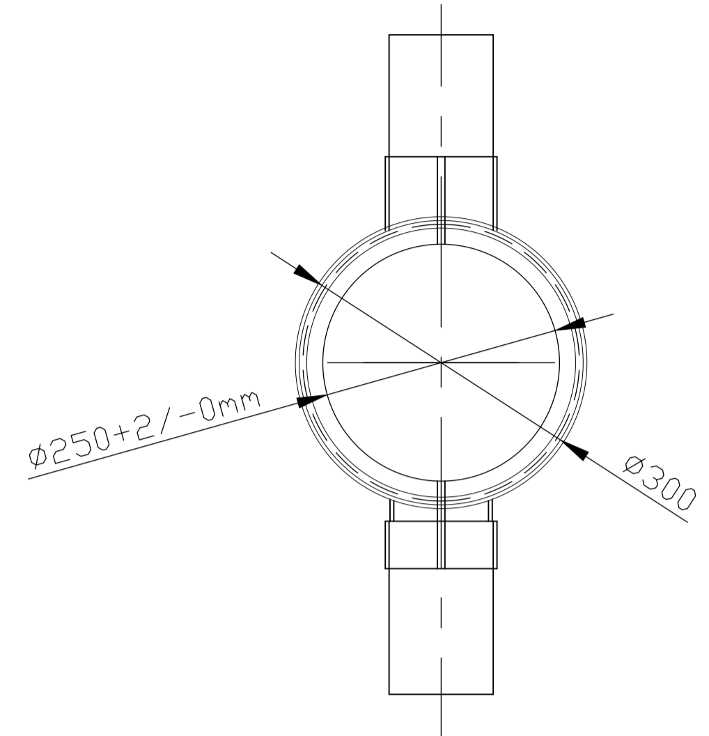
PLAN VIEW
