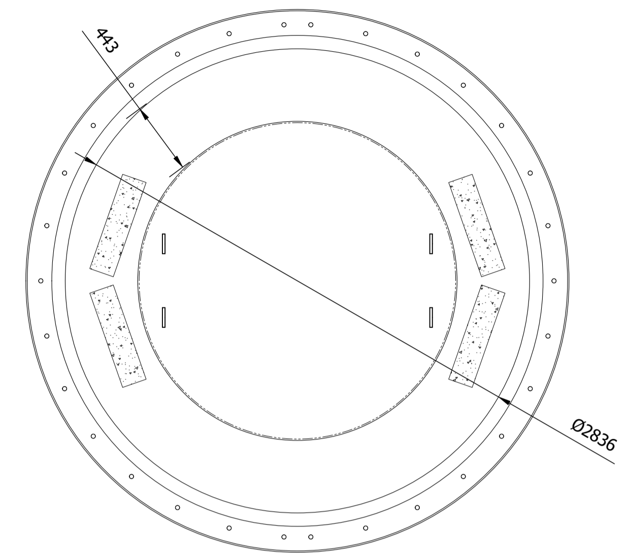
PLAN VIEW
