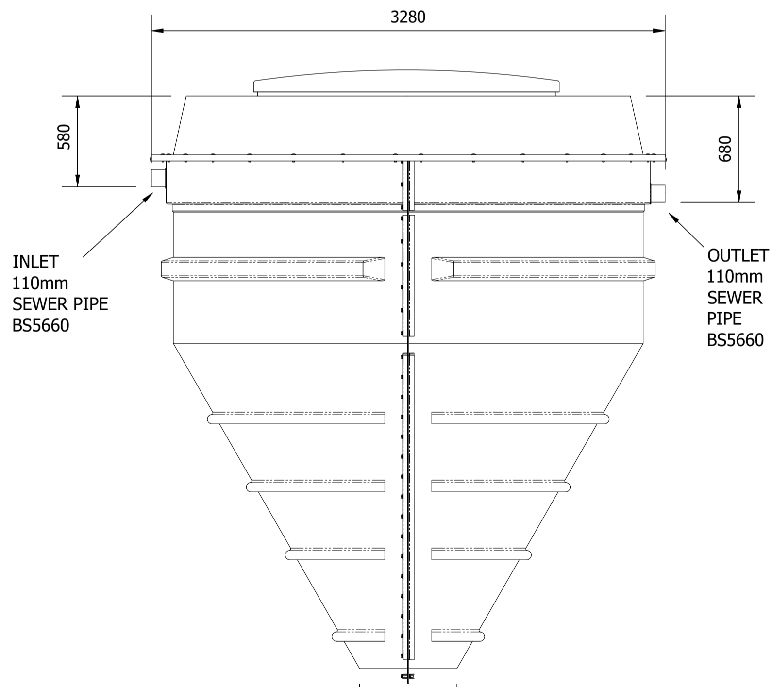
SIDE VIEW
