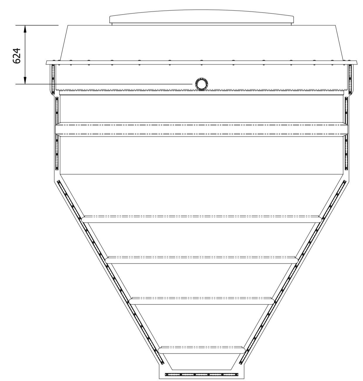
OUTLET VIEW
