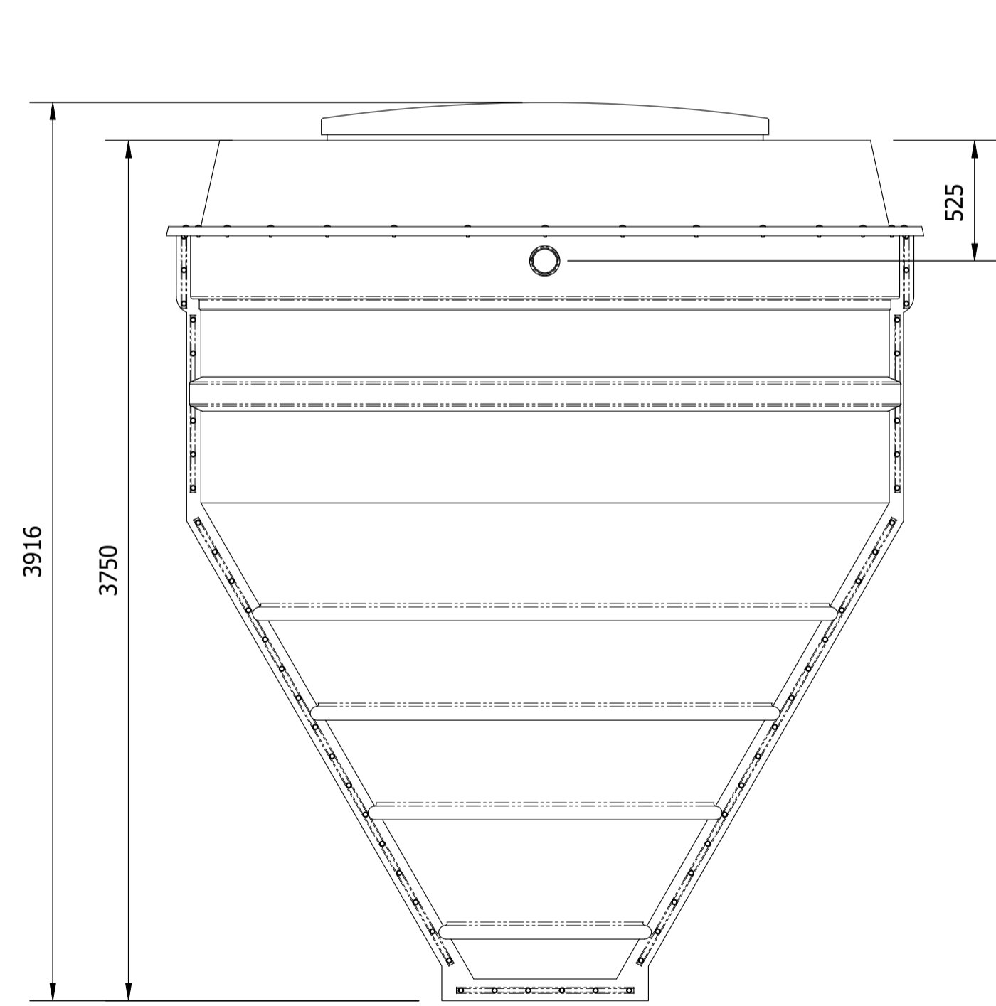
INLET VIEW
