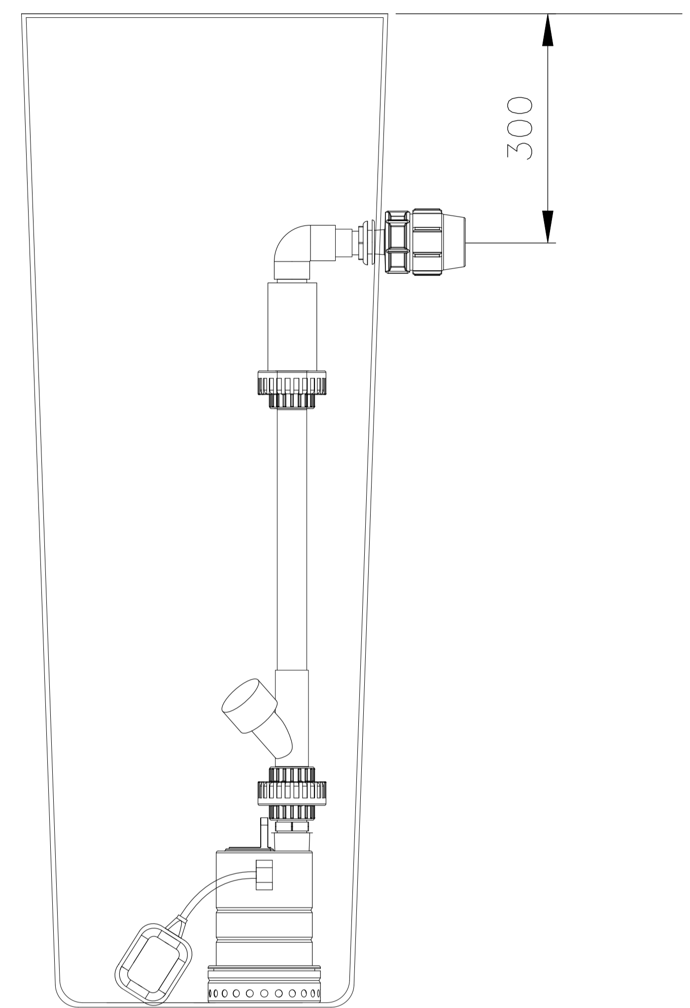
SECTION VIEW B-B
