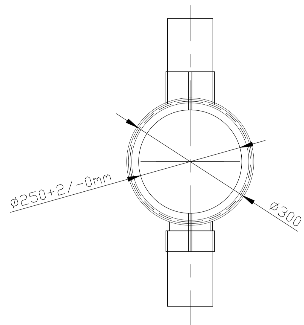
PLAN VIEW
