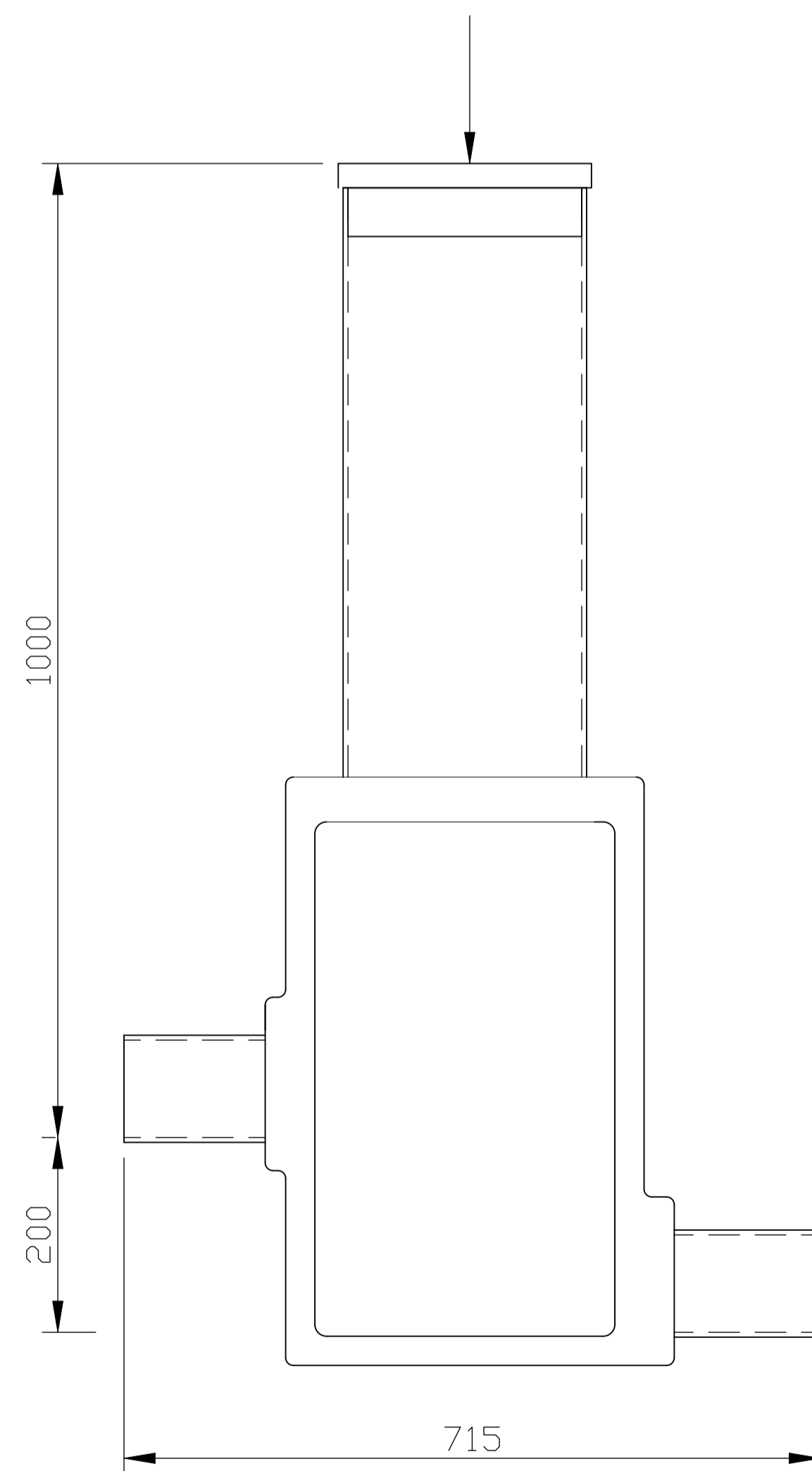
INSPECTION HATCH
